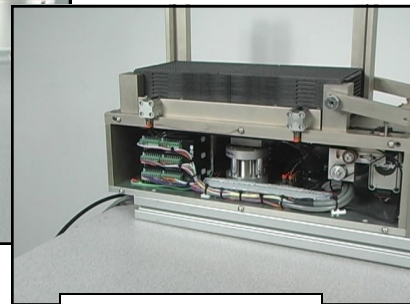
Un-stacker Internal
